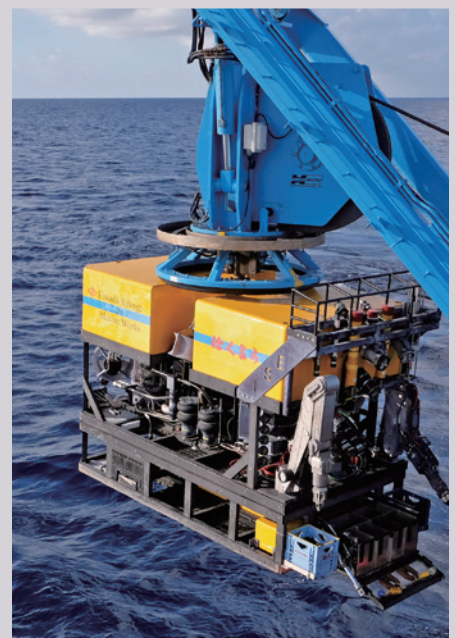
ROV HAKUYO Mother Vessel "SHIN NICHU MARU"
