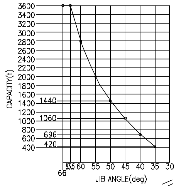
CAPACITY CURVE
