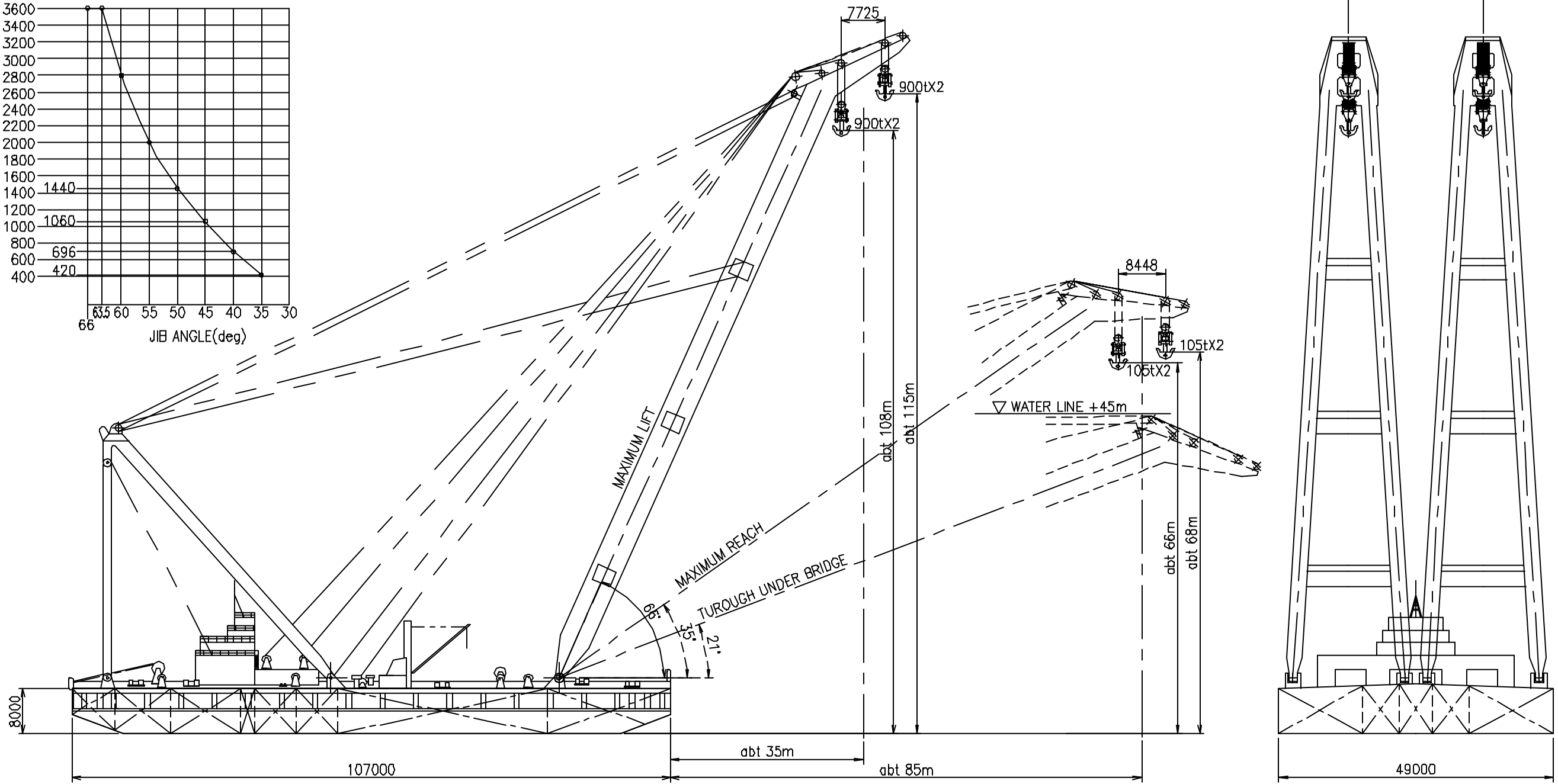
CAPACITY CURVE
