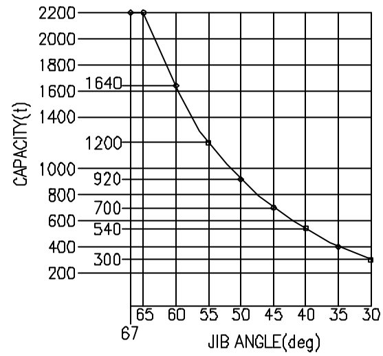
CAPACITY CURVE
