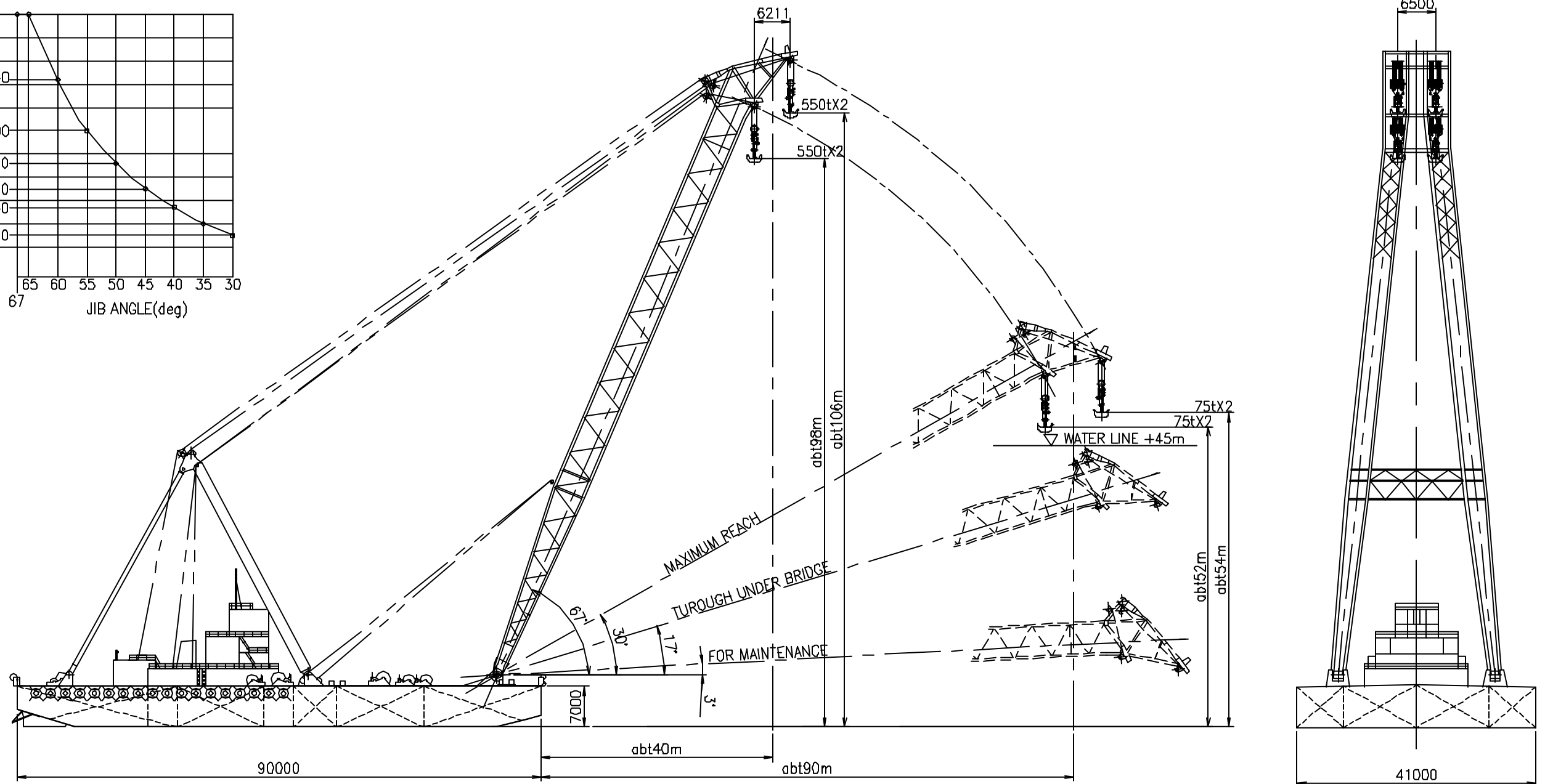
CAPACITY CURVE
